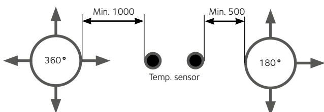
Forced ventilation diagram
